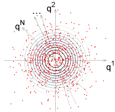
FIG. 2: Visualization of a generic distribution of N arbitrary properties, and its fitting by a generic Gaussian function. The coordinates q^3, \dots, q^N , extending along other dimensions, are orthogonal mutually and orthogonal to the depicted plane ( q^1, q^2 ).
